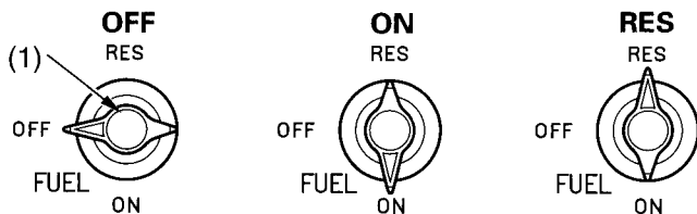
(1) fuel valve
